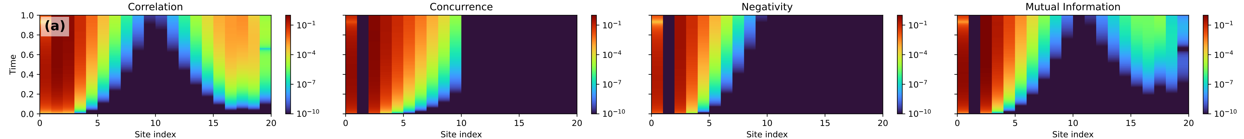
Product state (2,18) (band 2) - J_{long} = 20, J_z = 1, \alpha = 0.5
